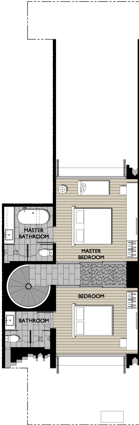
VILLA 2Br-A 2ND FLOOR PLAN
